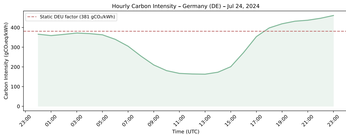
Figure 6.15: Hourly carbon intensity on 24 July 2024 in Germany
