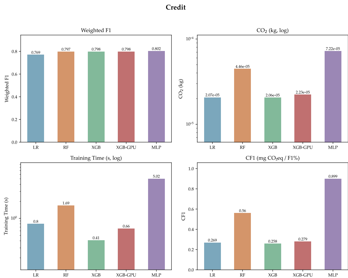
Figure C.2: Detailed benchmark results for the Credit Card Default dataset across all five models.
