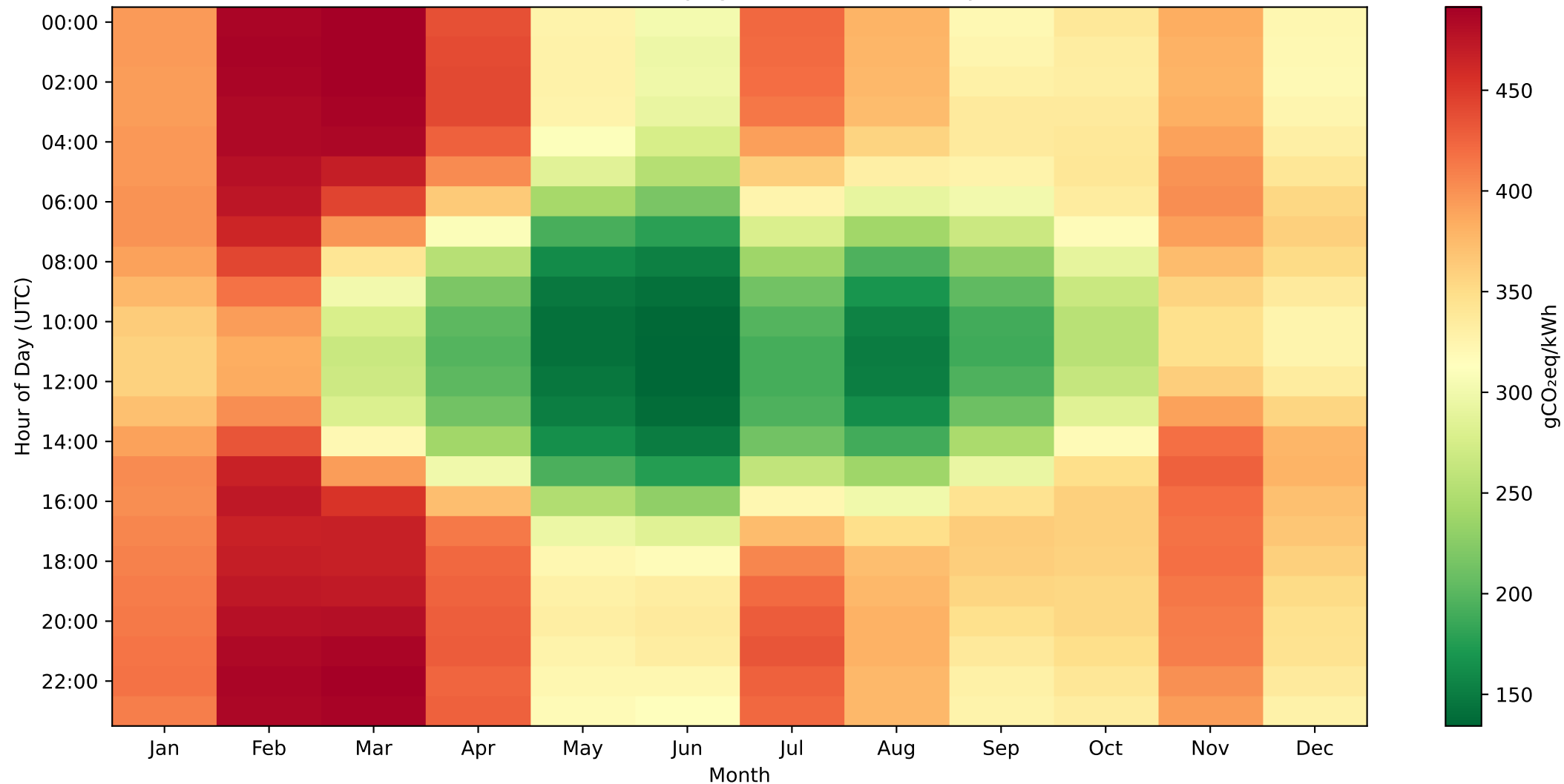
Mean Carbon Intensity (gCO 2 /kWh) - Germany 2025
