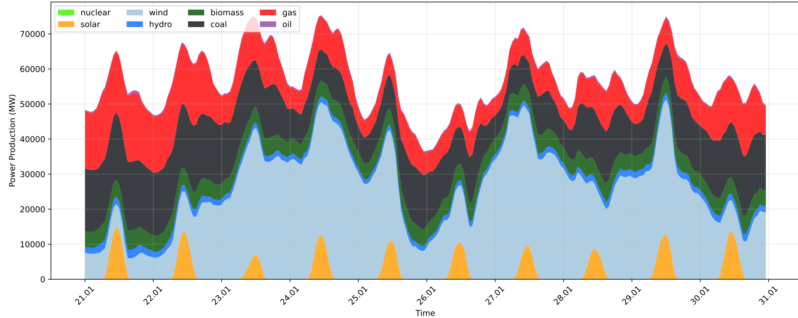
Electricity Mix - Germany (DE) - January
