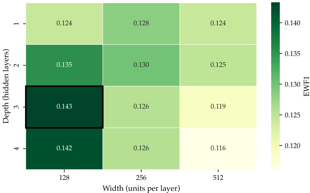
MLP Architecture Variation — EWF1 (HIGGS)
