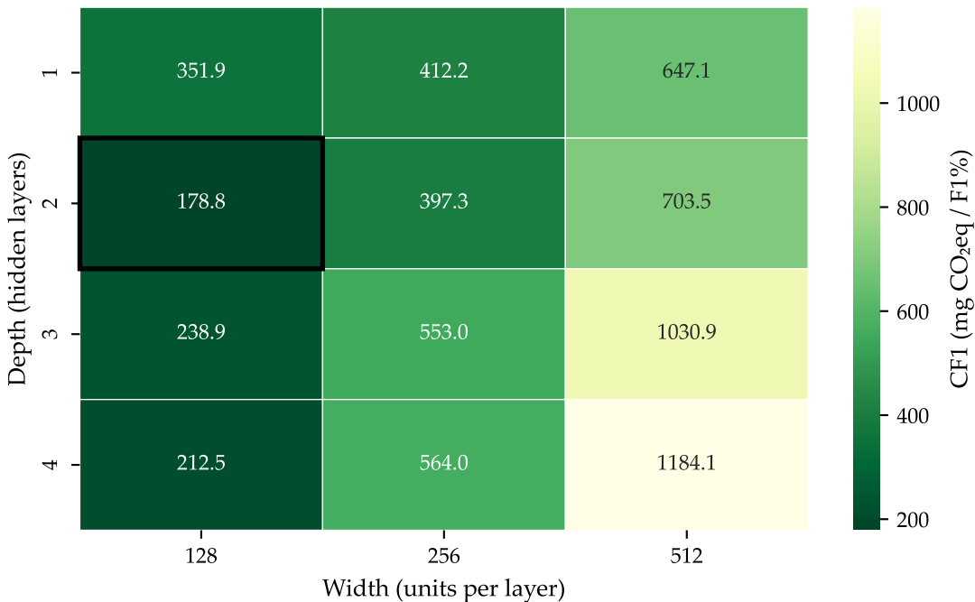
MLP Architecture Variation — CF1 (HIGGS)
