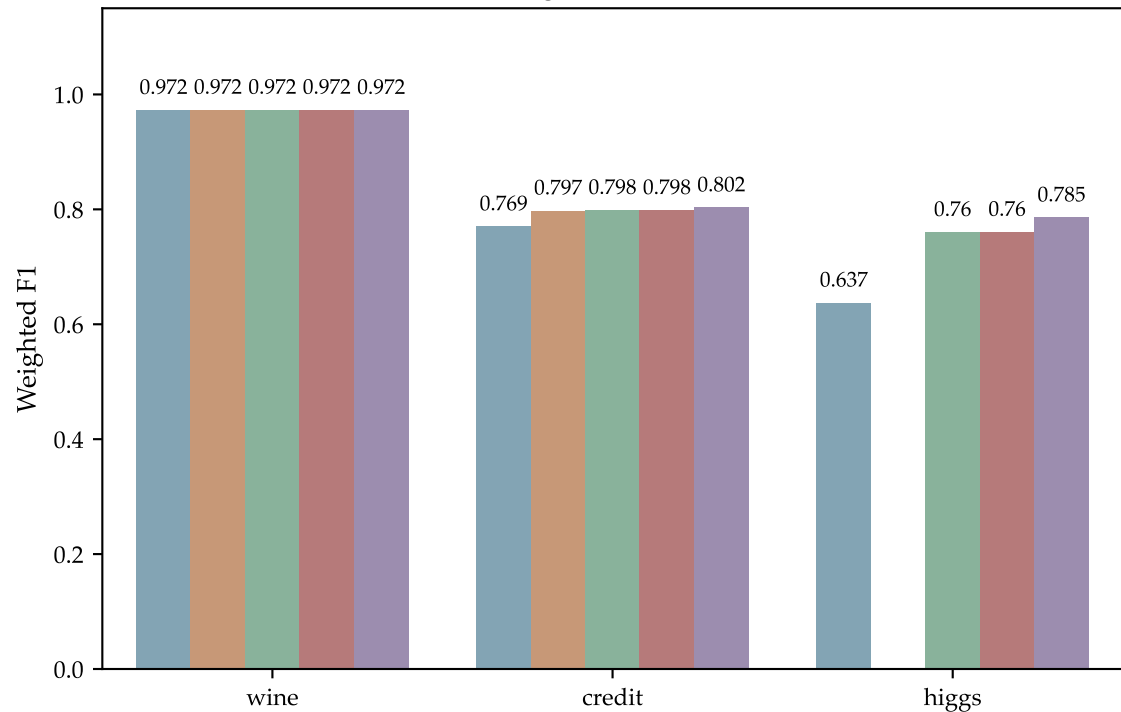
Weighted F1-Score
