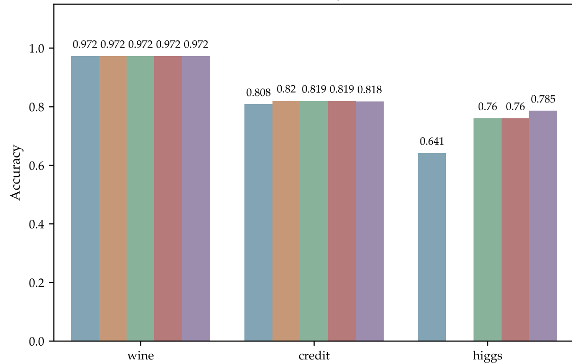
Accuracy
