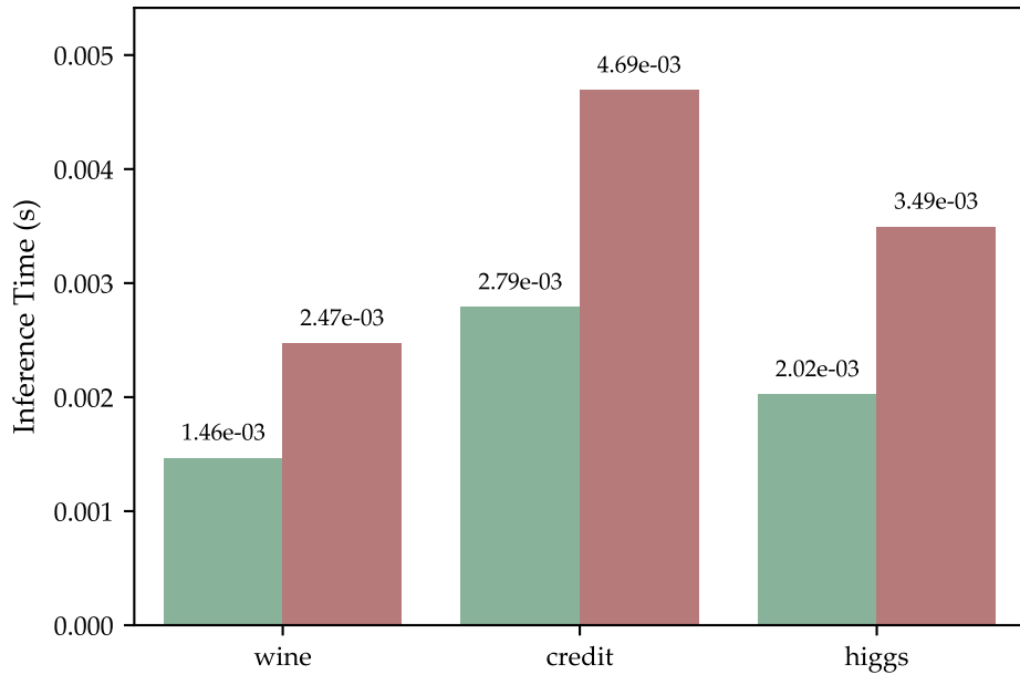
Inference Time
