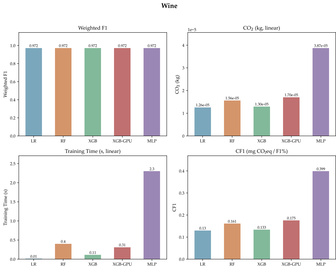
Figure C.1: Detailed benchmark results for the Wine dataset across all five models.
