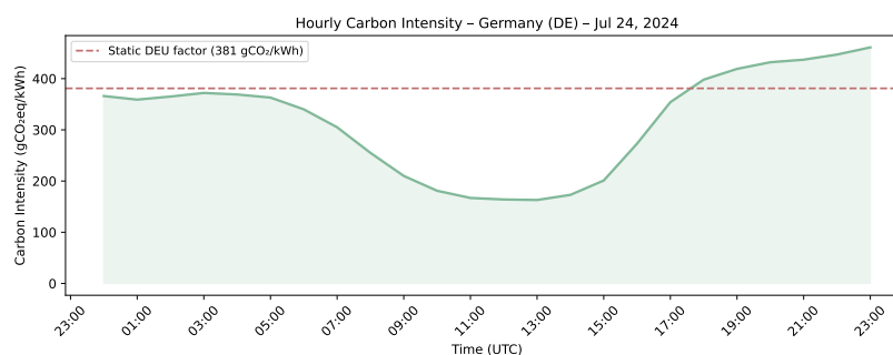
Figure 6.15: Hourly carbon intensity on 24 July 2024 in Germany
