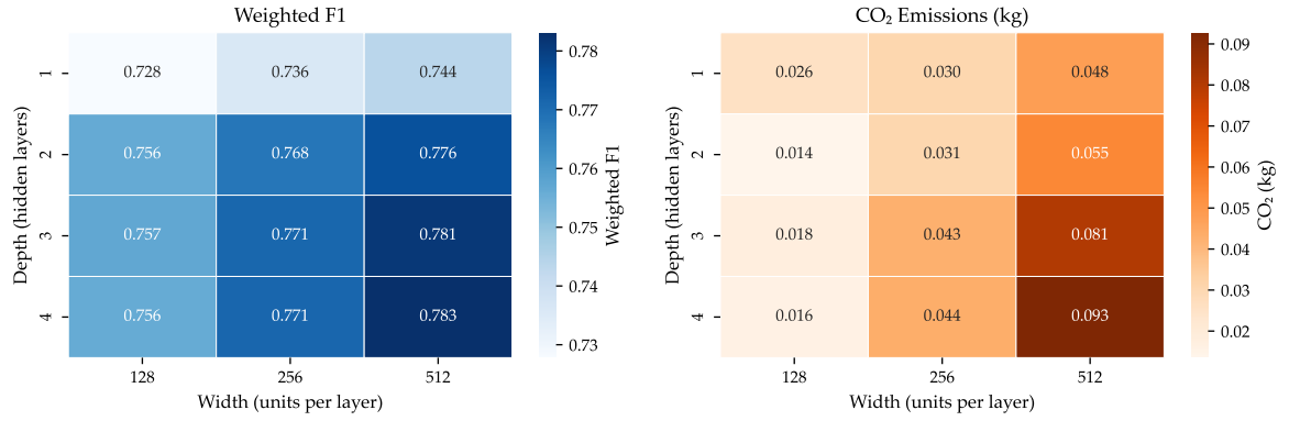
Figure 6.10: MLP architecture variation on HIGGS: weighted F1 (left) and CO 2 emissions (right) for all depth-width combinations. Darker cells indicate higher values.
