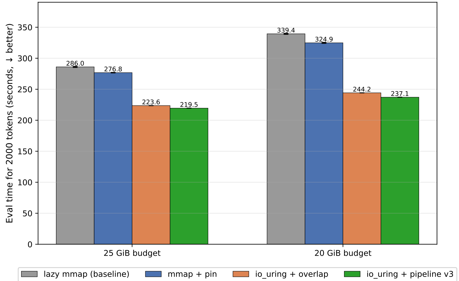
Eval time by configuration and budget (error bars = \sigma across iters)
