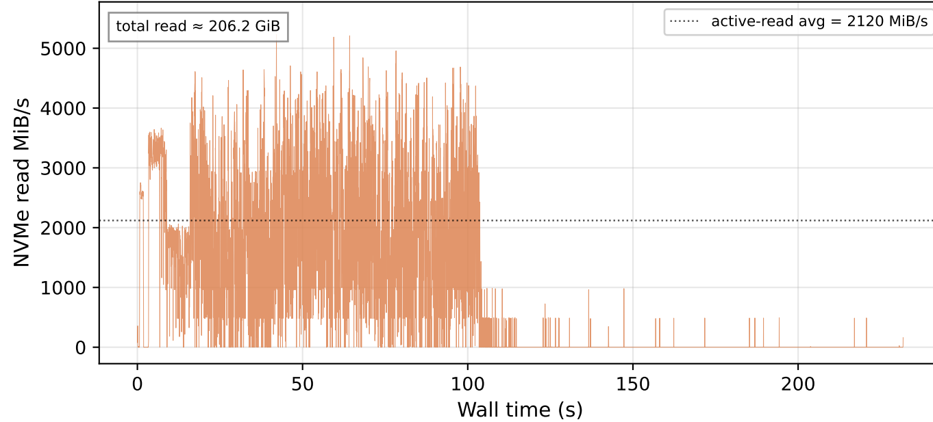
25 GiB — io_uring + overlap (raw 25 ms samples, 9014 points)
