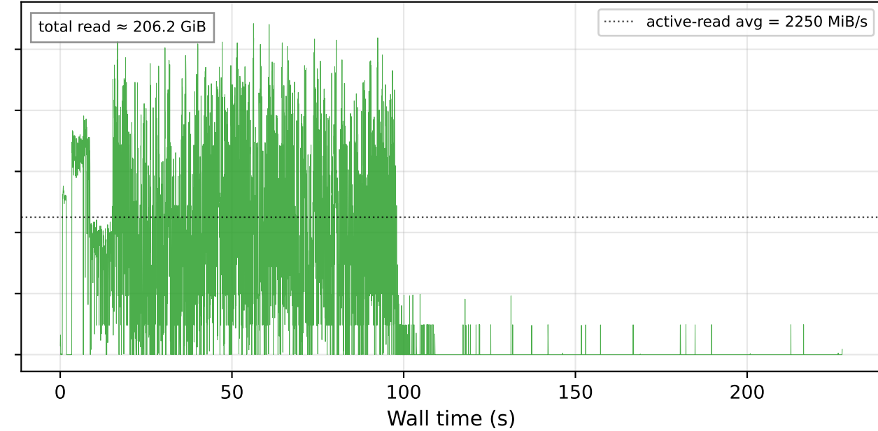
25 GiB — io_uring + pipeline v3 (raw 25 ms samples, 8852 points)
