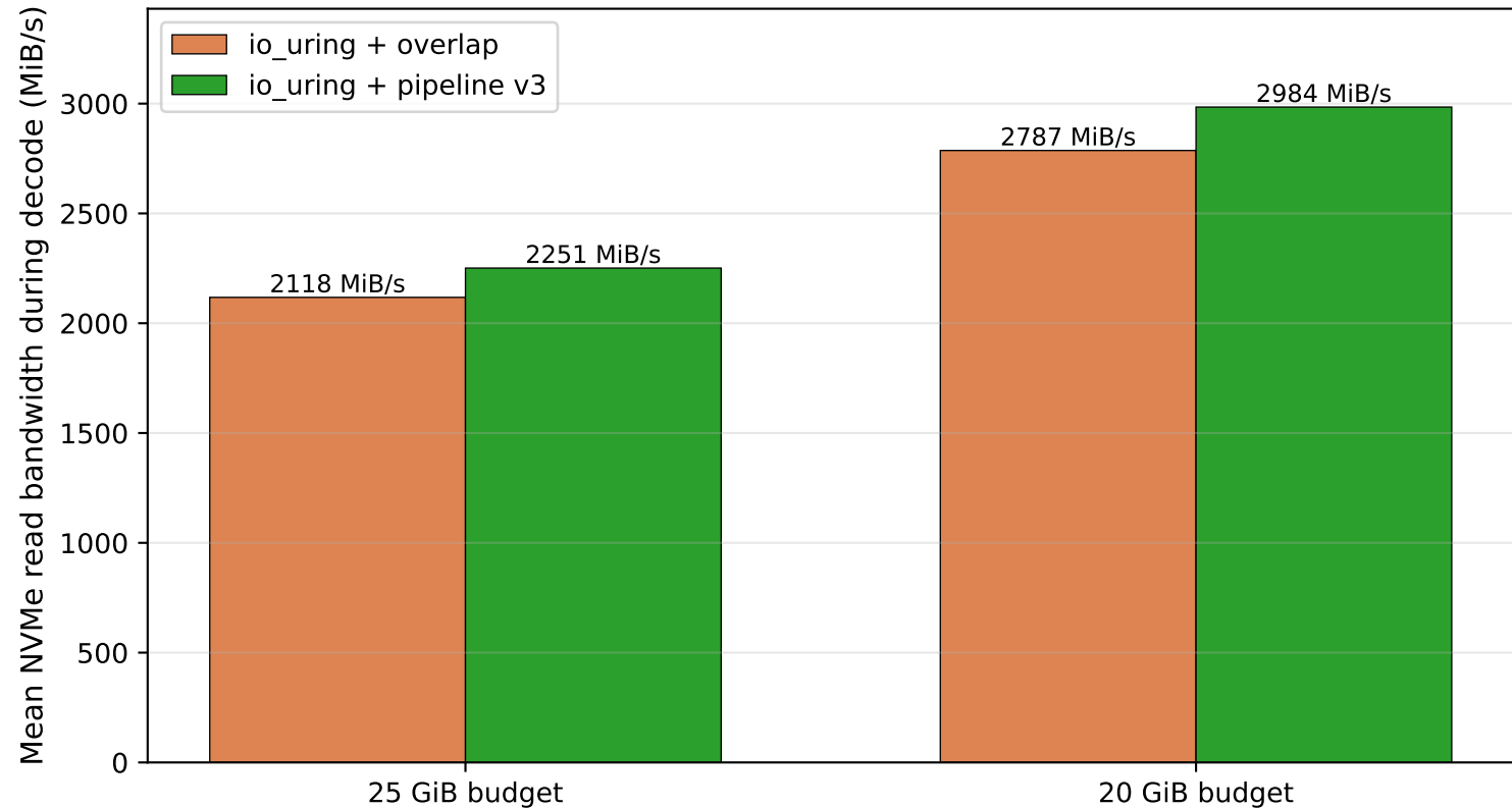
Sustained NVMe read bandwidth — v3 pulls more bytes per unit time
