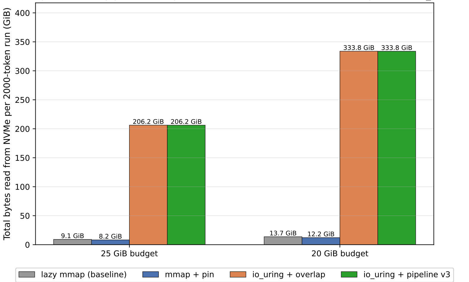
Disk I/O per run — lazy/pin via mmap faults (estimate: faults × 4 KiB); overlap/v3 from io_monitor
