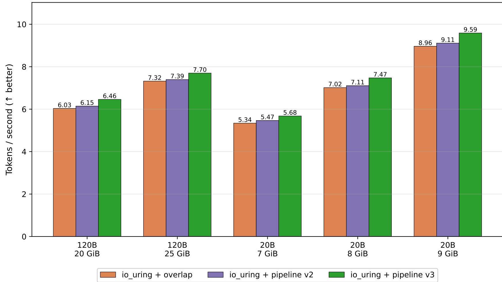
Decode throughput by pipeline mode, both models, all budgets — 3 iters, multi-topic prompt
