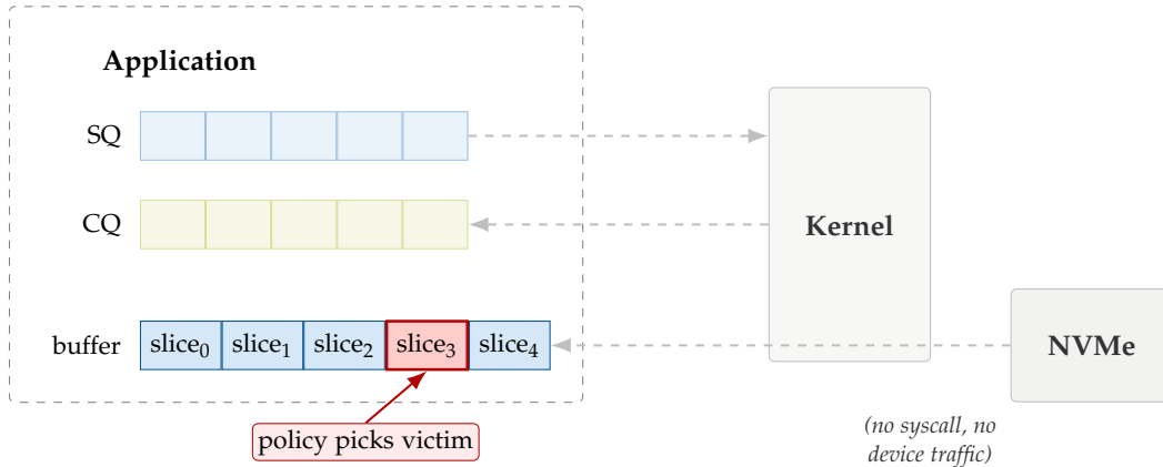
Figure 2.4.: Eviction step on a cache miss when the buffer is already full, drawn with the same building blocks as Figure 2.3. The application's replacement policy picks a victim slot (here slice3 , in red); no system call and no device traffic occur. The freed slot then serves as the DMA target for the read flow of Figure 2.3.
