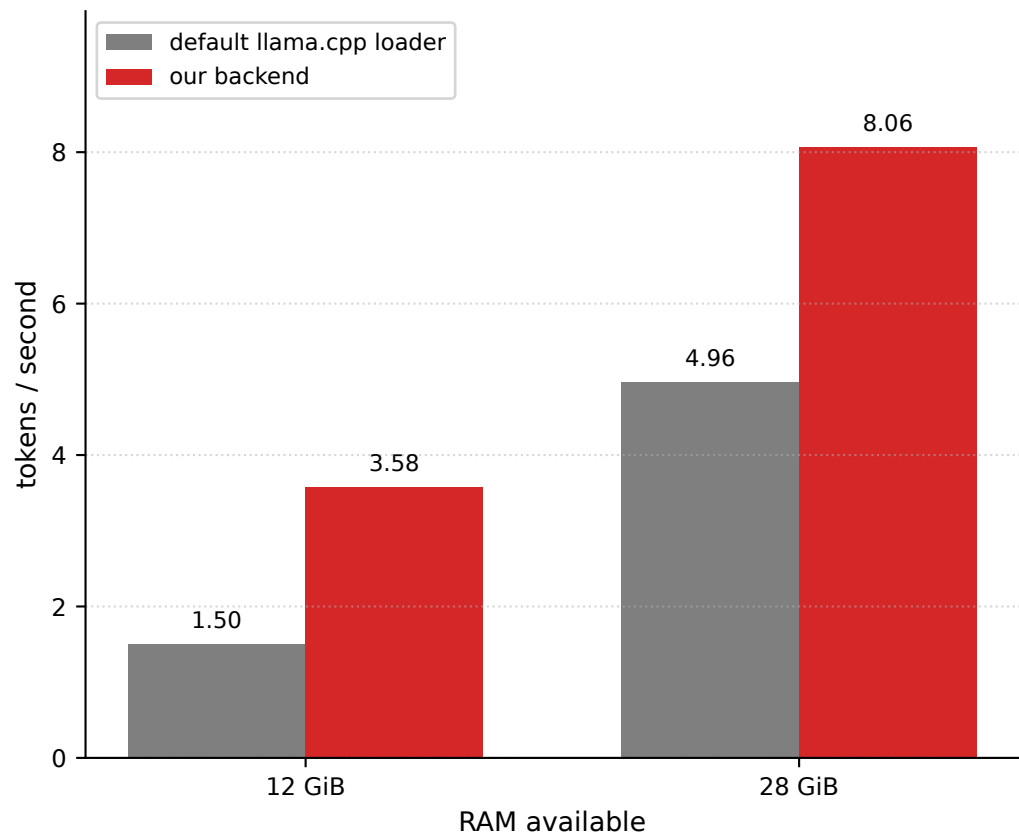
GPT-OSS-120B (61 GiB on disk, never fits in 30 GiB of RAM)
