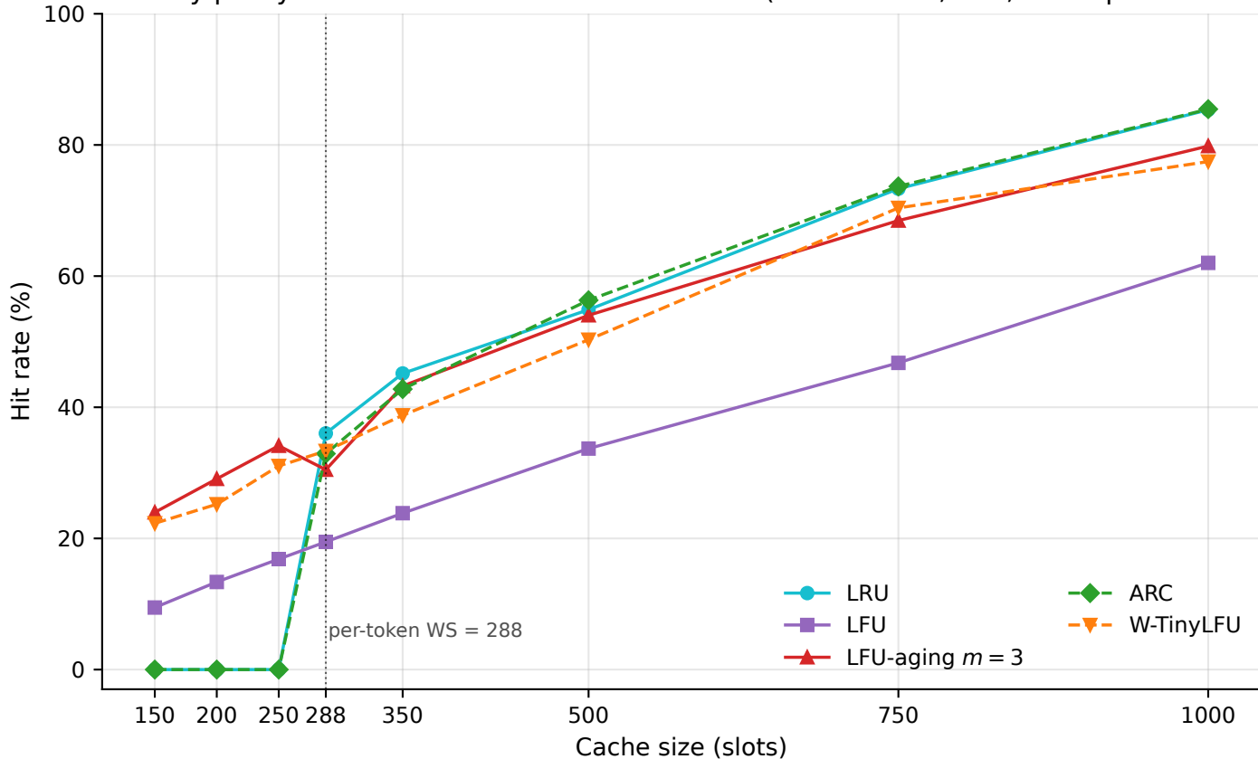
Hit rate by policy on the canonical 20B access trace (1999 tokens, 575,724 expert accesses)
