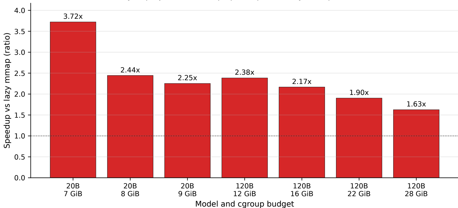
async-projection-overlap speedup over lazy mmap baseline
