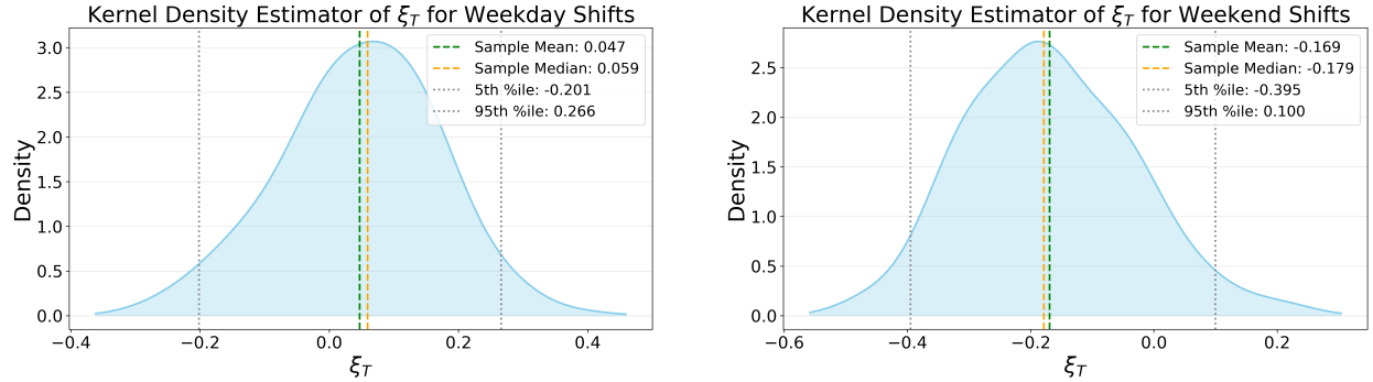
Figure 7: Kernel Density Estimator of the Last Period \xi_T
