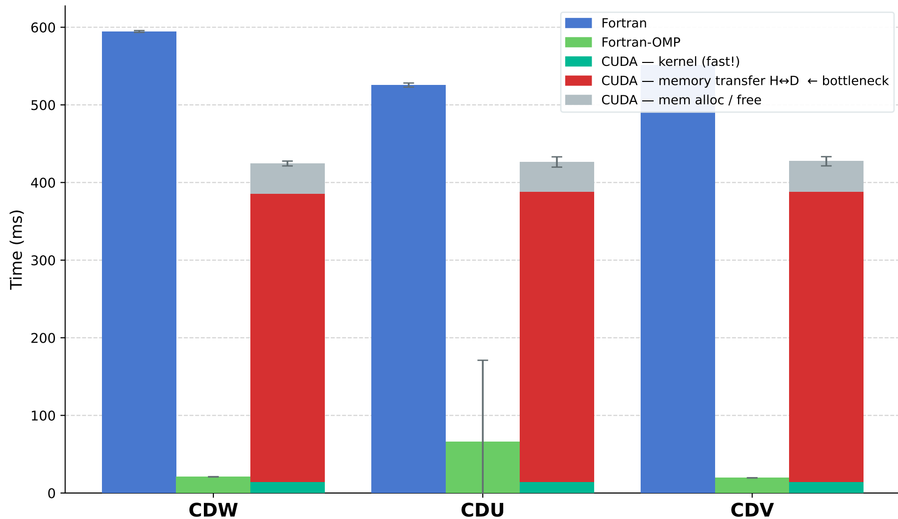
Benchmark comparison — grid 128×128×256, 50 iter/call
