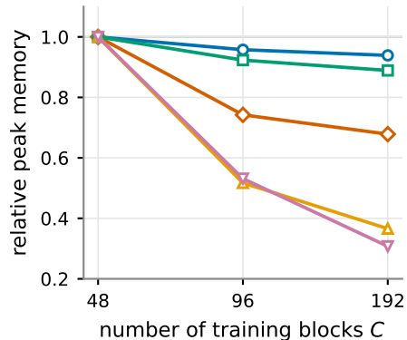
(c) inference memory vs. C
