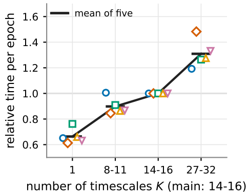
(a) training time vs. K
