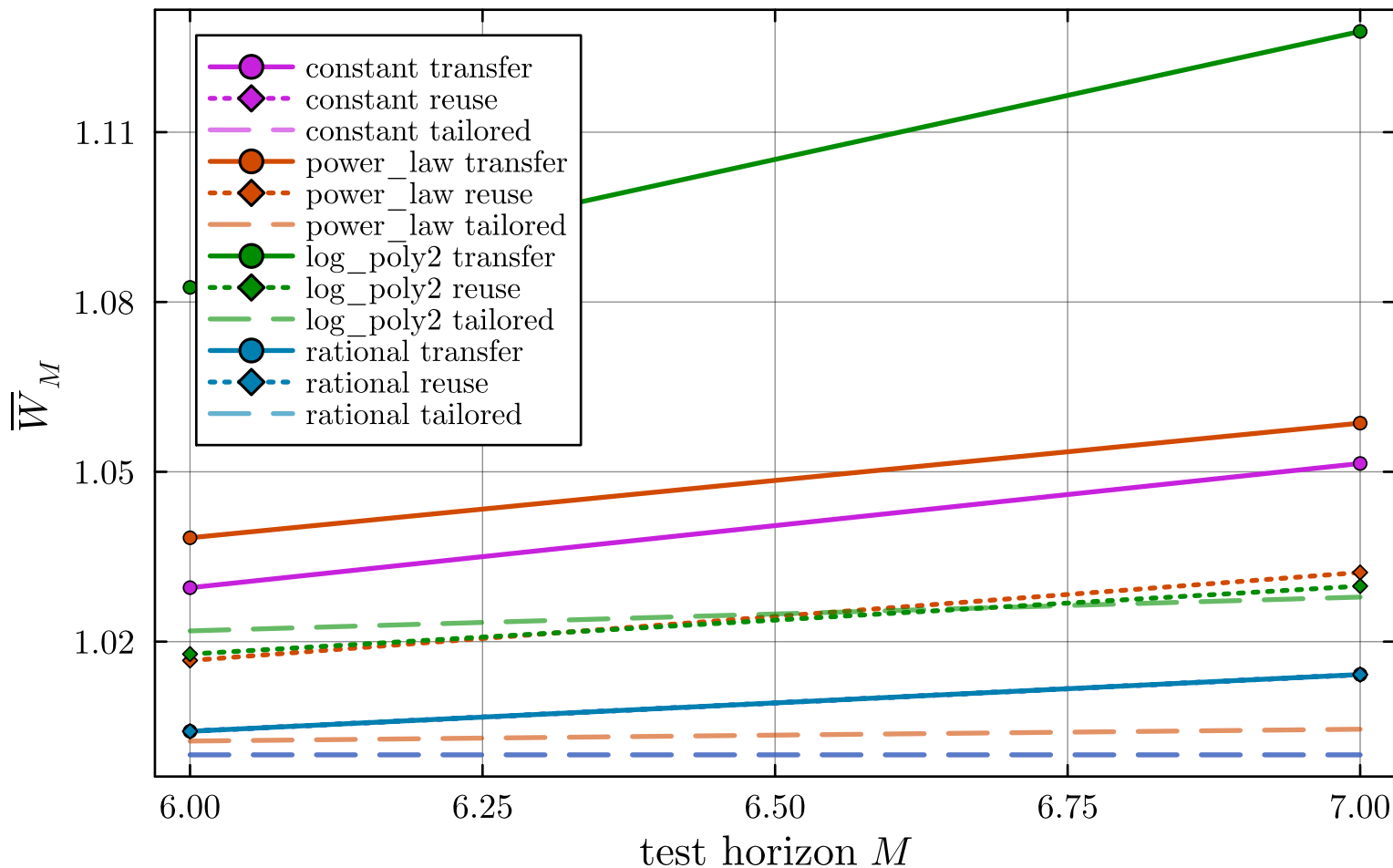
OGD anytime, train \leq 5
