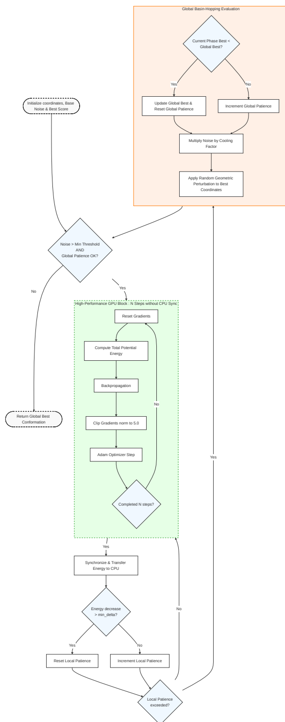
Figure 7: Overview of the combined local (Adam) and global (basin-hopping) optimization pipeline.
