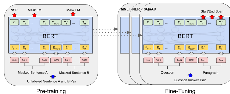
Figura 1.2: Pre-training e Fine-tuning BERT
