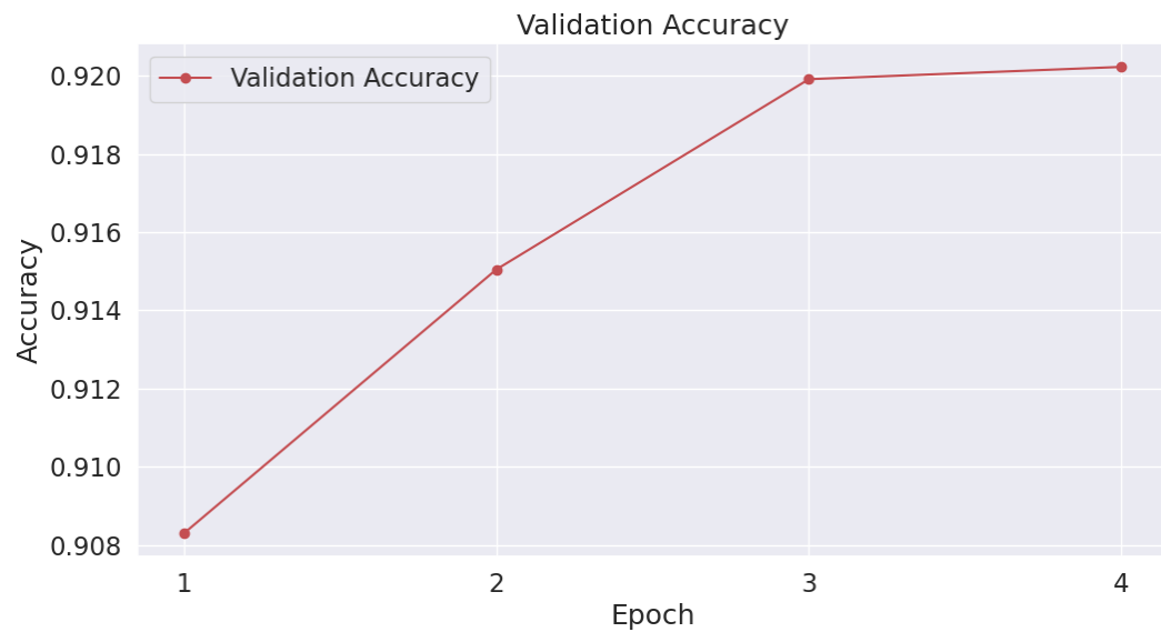
Figura 3.9: Validation accuracy
