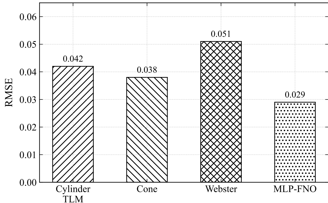
Рисунок 5 — RMSE comparison across methods
