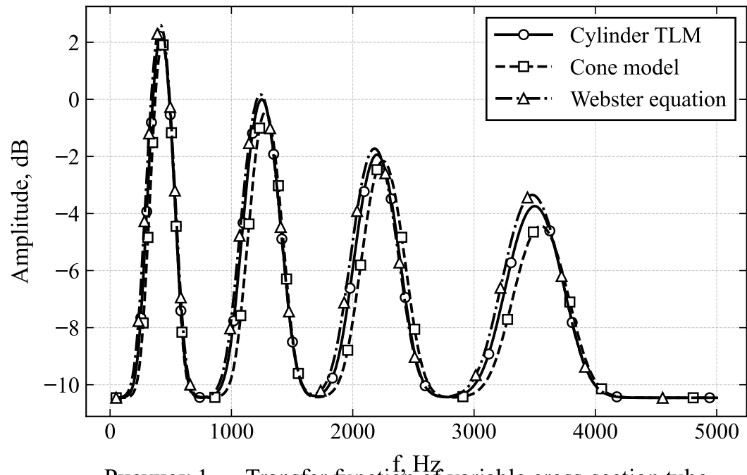
Рисунок 1 — Transfer function of variable cross-section tube
