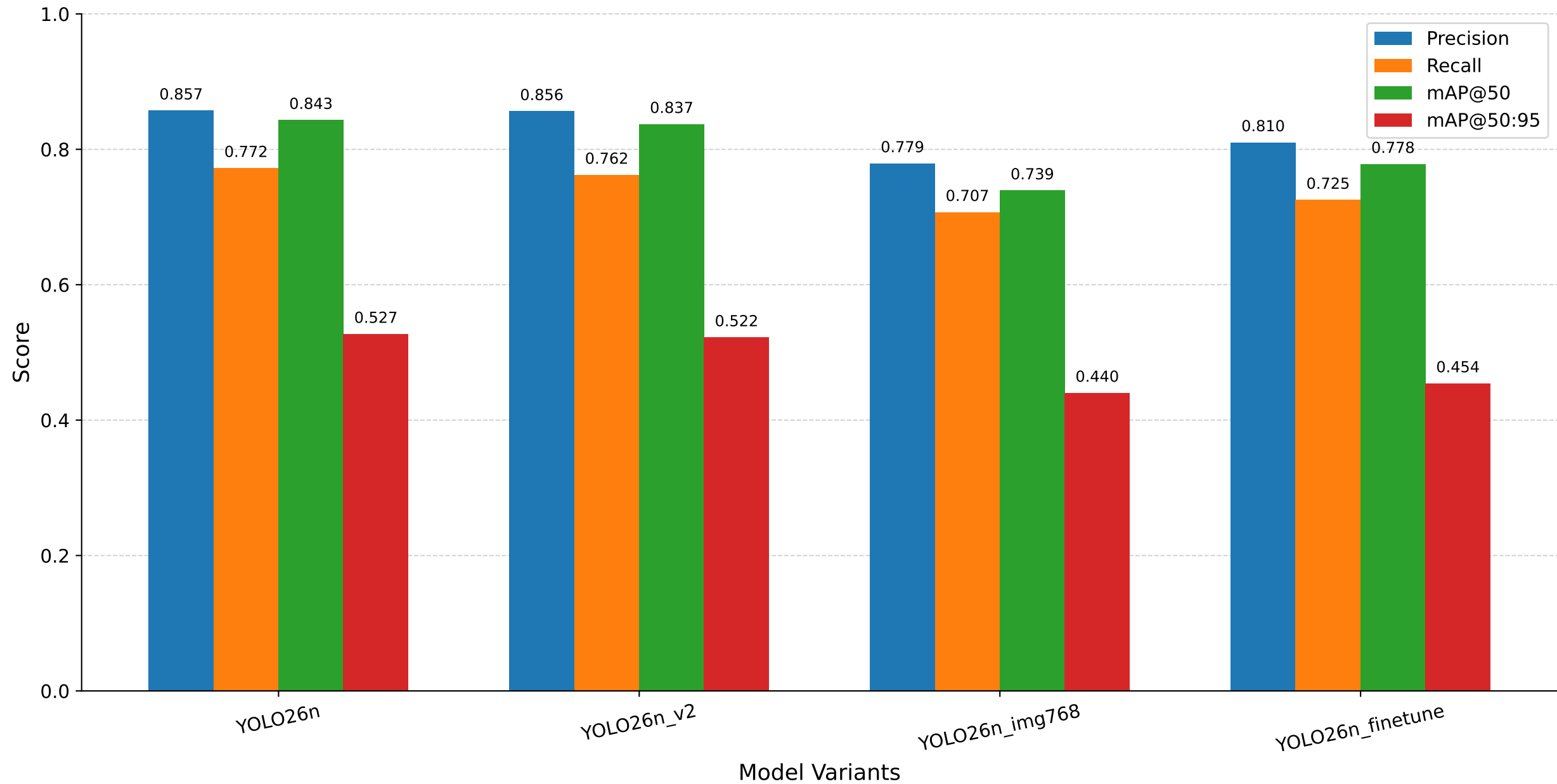
Performance Comparison of YOLO26n-Based Model Variants
