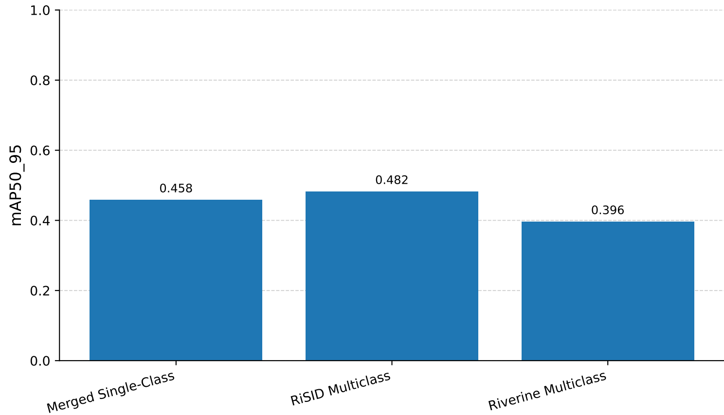
mAP50_95 Comparison Across YOLO26n Experiment Settings
