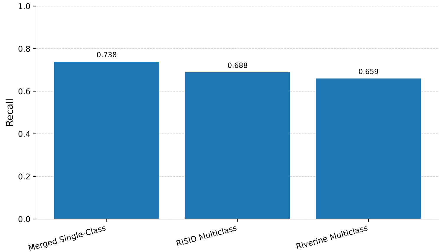
Recall Comparison Across YOLO26n Experiment Settings
