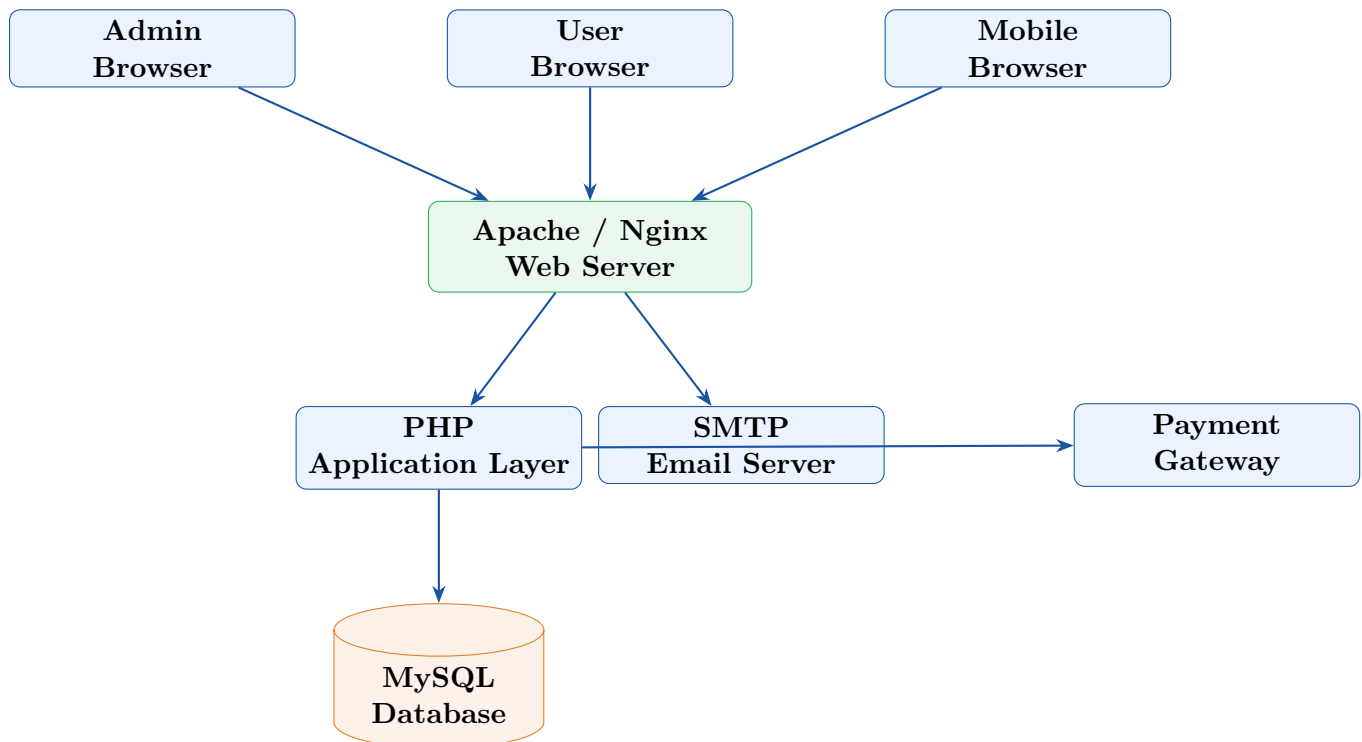
Figure 2.1: InternshipWala System Architecture Diagram
