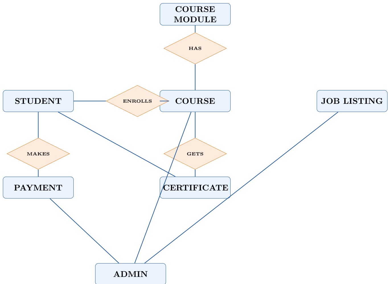
Figure 5.1: Simplified ER Diagram — InternshipWala
