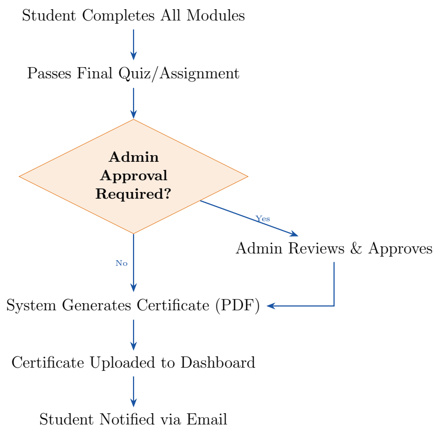
Figure 3.1: Certificate Generation Workflow
