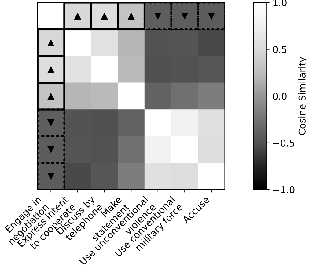
(b) With LLM Knowledge
