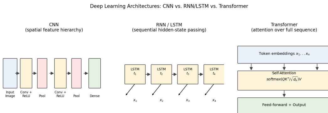
Figure 8.5: Three deep learning architectures compared. Left: a CNN builds up spatial features through alternating convolution and pooling layers. Middle: an RNN/LSTM processes a sequence one time step at a time, passing a hidden state forward. Right: a Transformer computes self-attention over the entire input sequence at once, letting every token directly attend to every other token.
