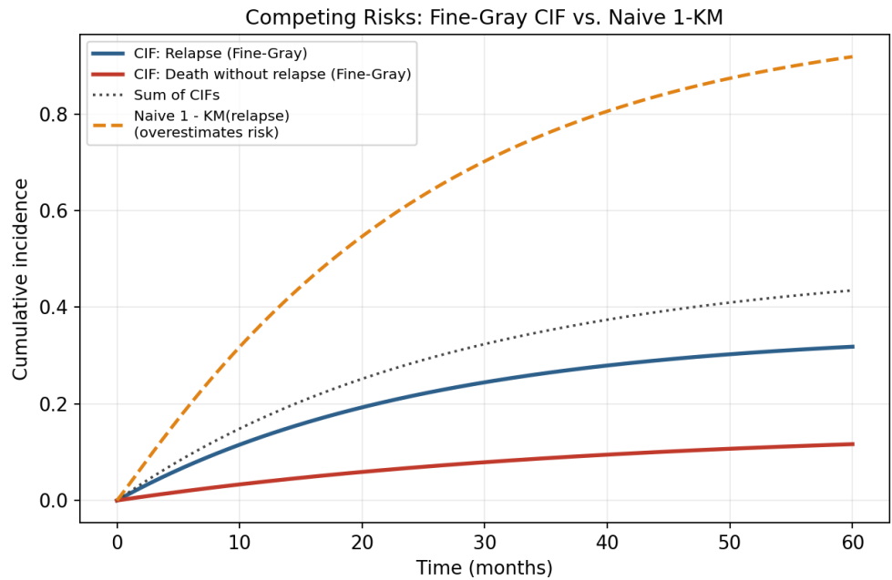
Figure 4.4: Cumulative incidence functions under competing risks. Fine-Gray CIFs for relapse (blue) and death without relapse (red) sum to the total event probability (dotted grey); the naive “1 minus Kaplan-Meier” curve for relapse (orange dashed), which incorrectly treats death as simple censoring, visibly overestimates the true relapse risk.
