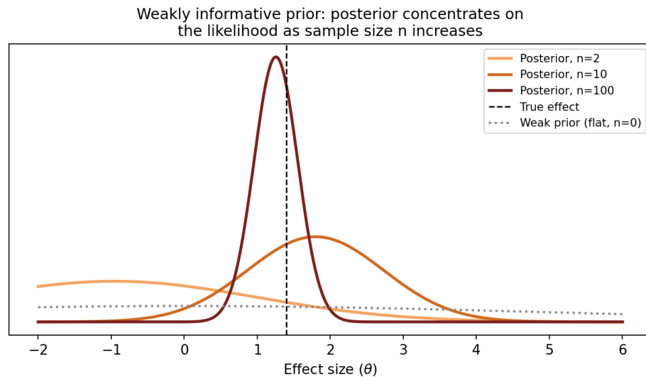
Figure 2.2: A weakly informative prior is dominated by the likelihood as sample size grows. The dotted grey curve shows a deliberately vague (weak) prior centered at zero. The three colored curves show the resulting posterior distribution for the same underlying effect at increasing sample sizes ( n=2, 10, 100 ), holding the prior fixed.
