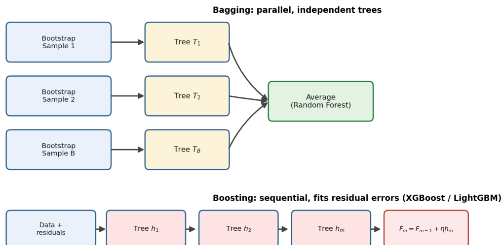
Figure 8.4: Bagging versus boosting. Top: Random Forest (bagging) fits B trees independently and in parallel to different bootstrap samples, then averages their predictions. Bottom: gradient boosting (XGBoost/LightGBM) fits trees sequentially, with each new tree specifically targeting the residual error left by the previous ensemble.
