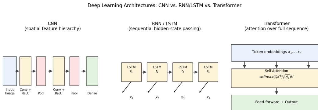
Figure 10.5: Three deep learning architectures compared. Left: a CNN builds up spatial features through alternating convolution and pooling layers. Middle: an RNN/LSTM processes a sequence one time step at a time, passing a hidden state forward. Right: a Transformer computes self-attention over the entire input sequence at once, letting every token directly attend to every other token.
