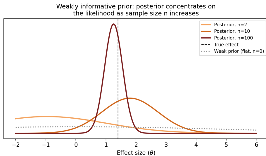
Figure 3.2: A weakly informative prior is dominated by the likelihood as sample size grows. The dotted grey curve shows a deliberately vague (weak) prior centered at zero. The three colored curves show the resulting posterior distribution for the same underlying effect at increasing sample sizes ( n=2, 10, 100 ), holding the prior fixed.
