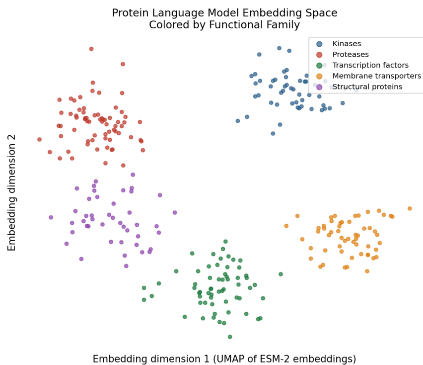
Figure 8.2: Protein embedding space colored by functional family. A two-dimensional projection (e.g., UMAP) of ESM-2 embeddings for a diverse set of proteins, colored by known functional annotation.
