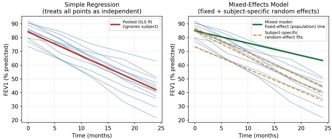
Figure 3.3: Mixed-effects models versus simple regression for longitudinal data. Simulated FEV1 trajectories for 12 patients measured at five clinic visits over 24 months. Left: a simple (pooled) regression line fit by ordinary least squares, treating all 60 observations as independent. Right: a mixed-effects model, showing the fixed-effect (population-average) line in green together with three example subject-specific fitted trajectories (dashed orange), each incorporating that patient’s own random intercept and slope.
