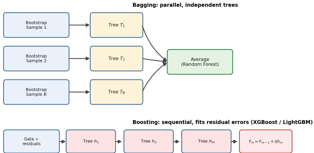
Figure 10.4: Bagging versus boosting. Top: Random Forest (bagging) fits B trees independently and in parallel to different bootstrap samples, then averages their predictions. Bottom: gradient boosting (XGBoost/LightGBM) fits trees sequentially, with each new tree specifically targeting the residual error left by the previous ensemble.
