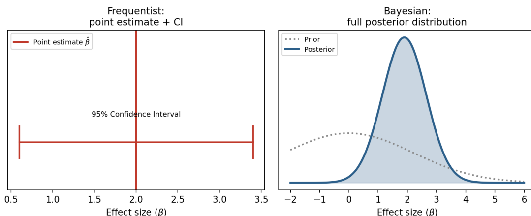
Figure 3.1: Frequentist versus Bayesian representations of the same estimated effect. Left: the frequentist output is a single point estimate ( \hat{\beta} ) with a 95% confidence interval, computed from the sampling distribution of the estimator. Right: the Bayesian output is a full posterior probability distribution over the effect size, obtained by updating a prior with the likelihood of the observed data.
