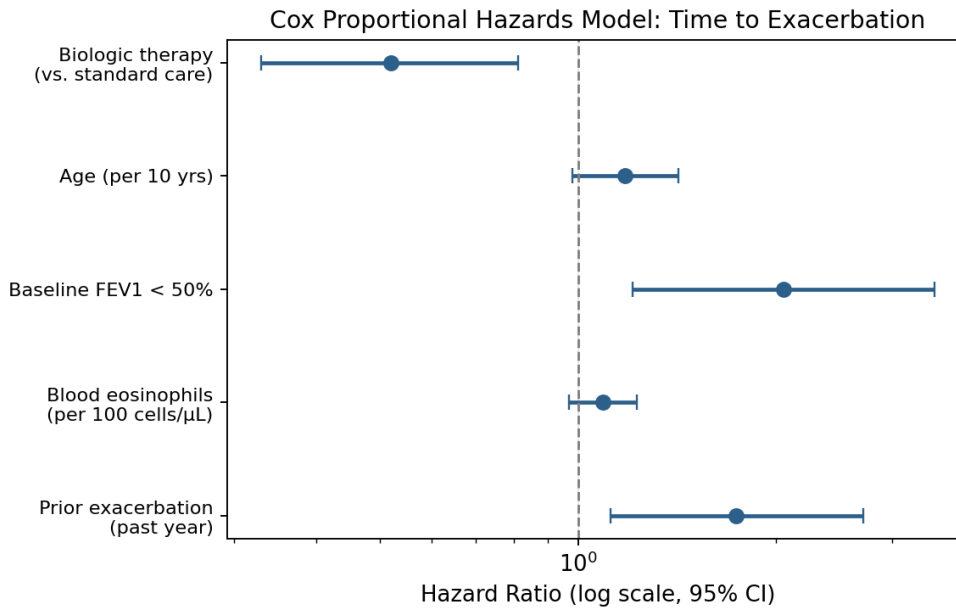
Figure 4.2: Cox model forest plot. Hazard ratios (points) and 95% confidence intervals (error bars) for five covariates in a model of time to severe asthma exacerbation, plotted on a log scale. The vertical dashed line at HR=1 marks no effect.
