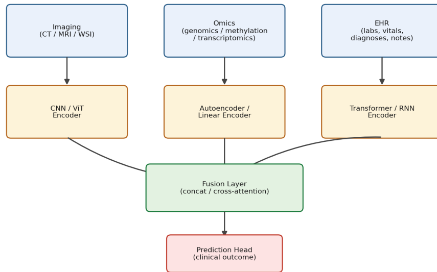
Figure 10.3: Intermediate/joint multimodal fusion architecture. Each modality (imaging, omics, EHR) is first passed through its own encoder to produce a fixed-length embedding; the three embeddings are then combined in a fusion layer (concatenation or cross-attention) before a shared prediction head produces the final clinical output.
