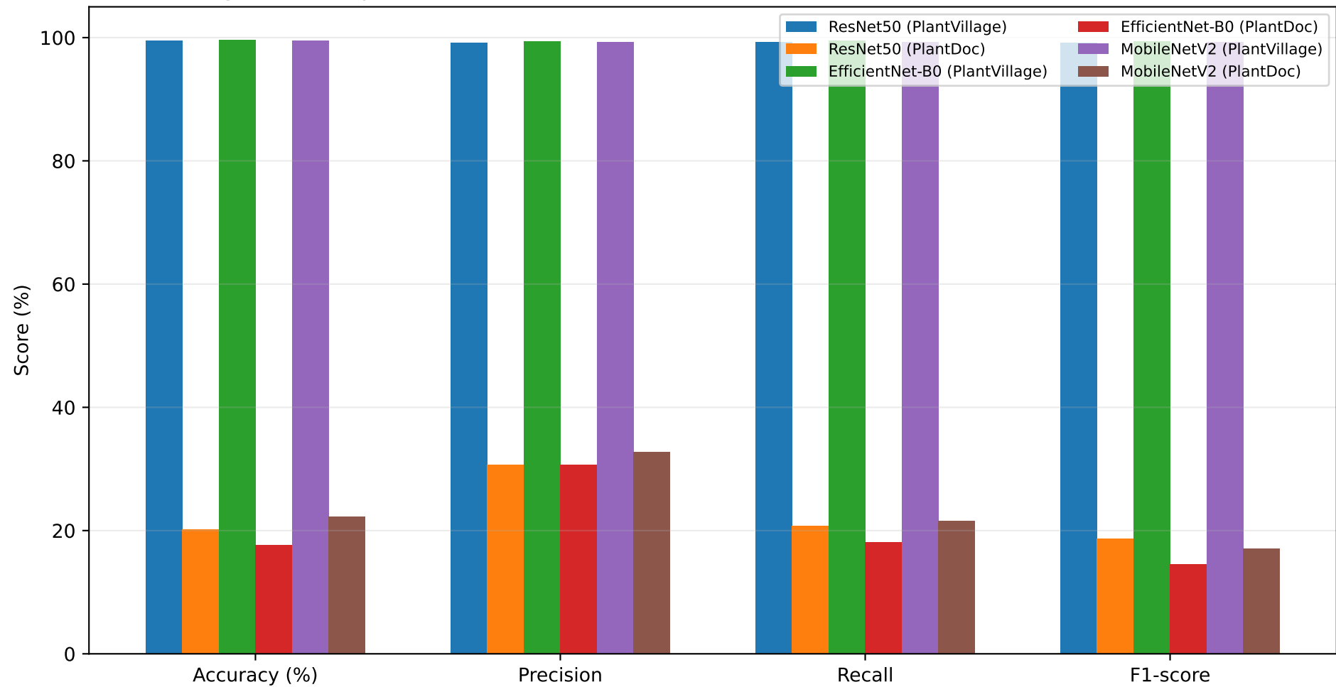
Figure 1. Comparative Performance of CNN Architectures Under Cross-Dataset Evaluation
