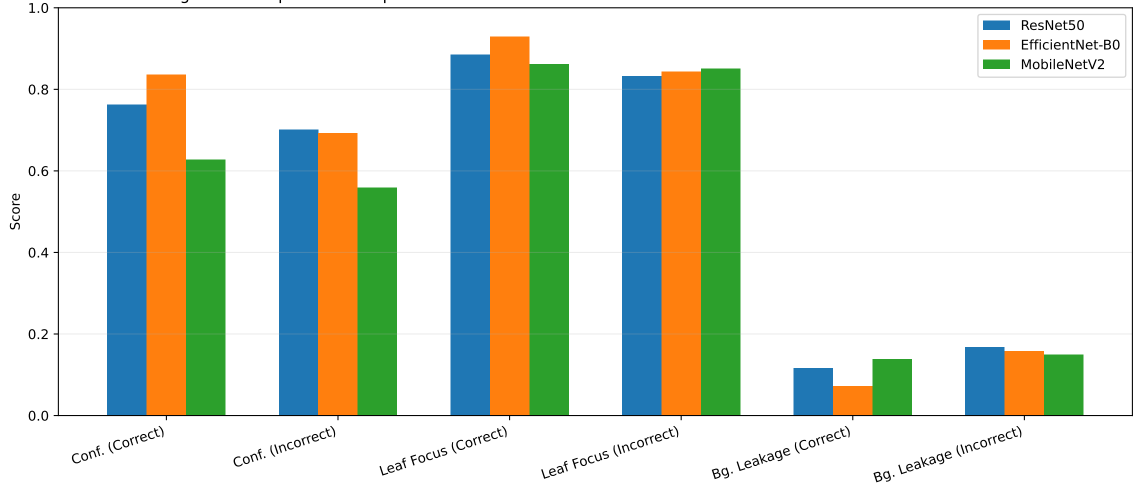
Figure 8. Comparison of Explanation Behavior in Correct and Incorrect Predictions Across Backbone Models
