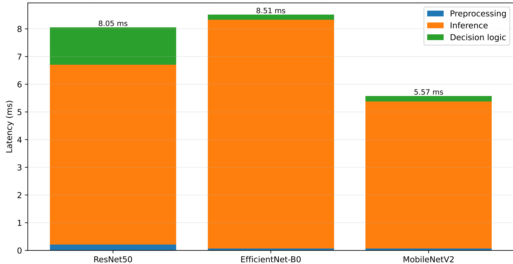
Figure 10. Measured Deployment Pipeline Latency Breakdown Across Models
