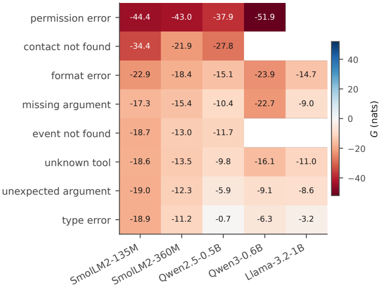
Corrective gain by error family
