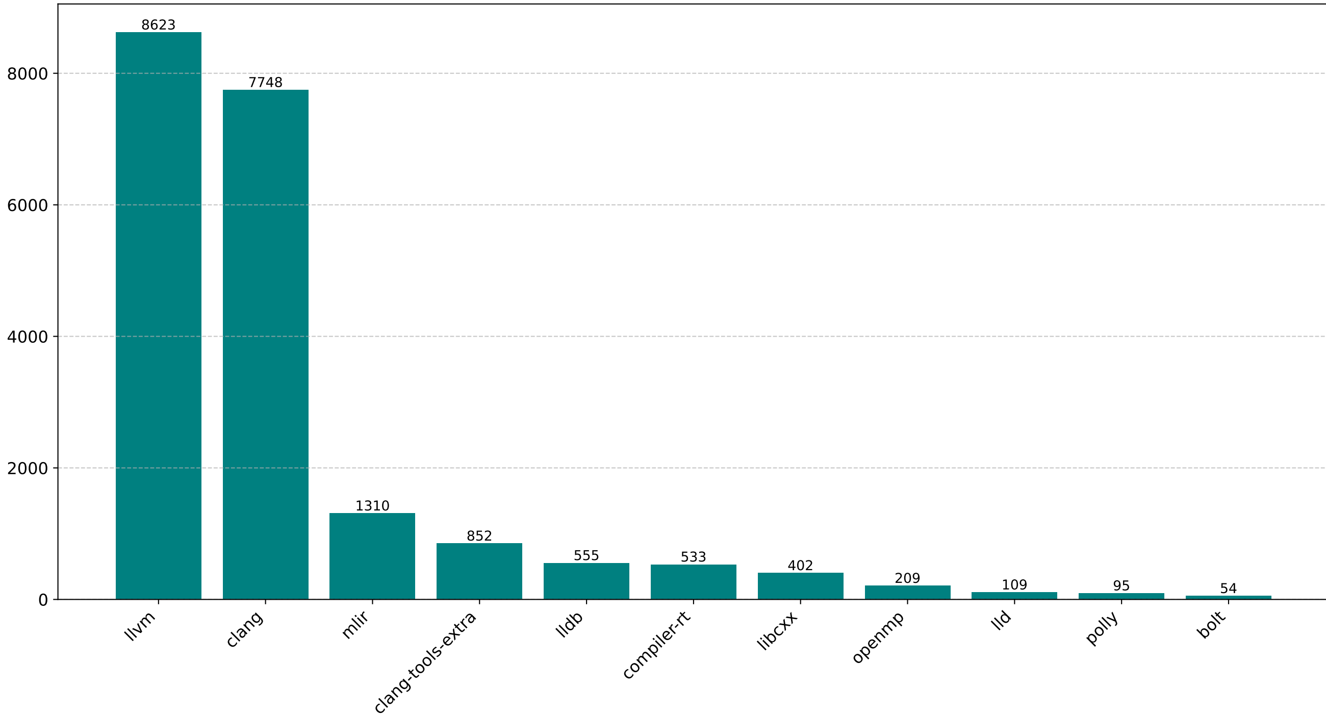
SATD Distribution in LLVM Project Modules
