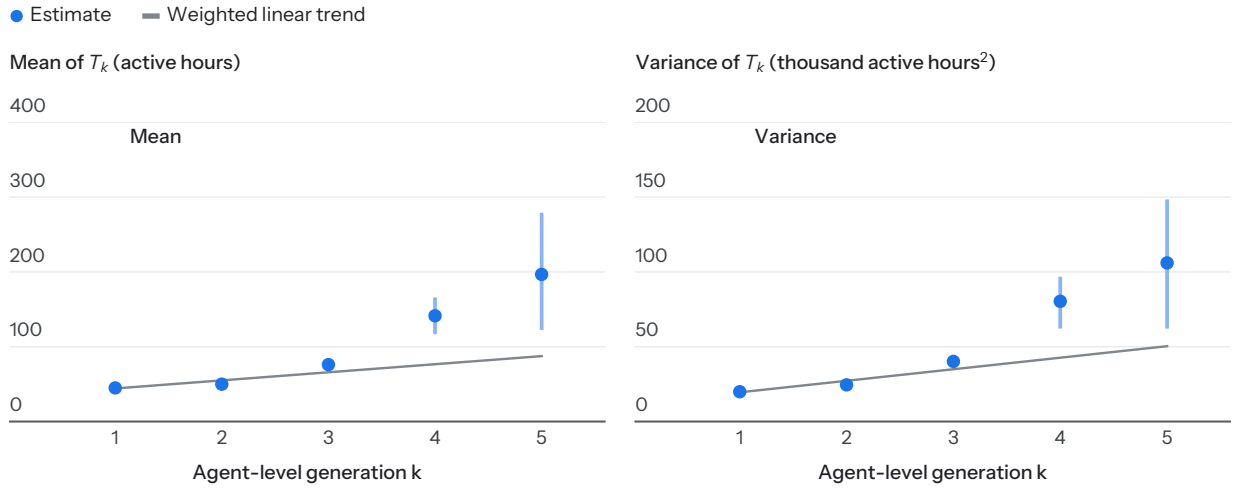
Figure 10: Mean and variance of T_k , the active time from a tree root to an acquisition at agent-level generation k on the MAP forest. Intervals are root-cluster bootstrap 95% intervals, and the line is the weighted linear trend in k . From k = 3 on, both estimates and their whole intervals lie above the linear trend.
