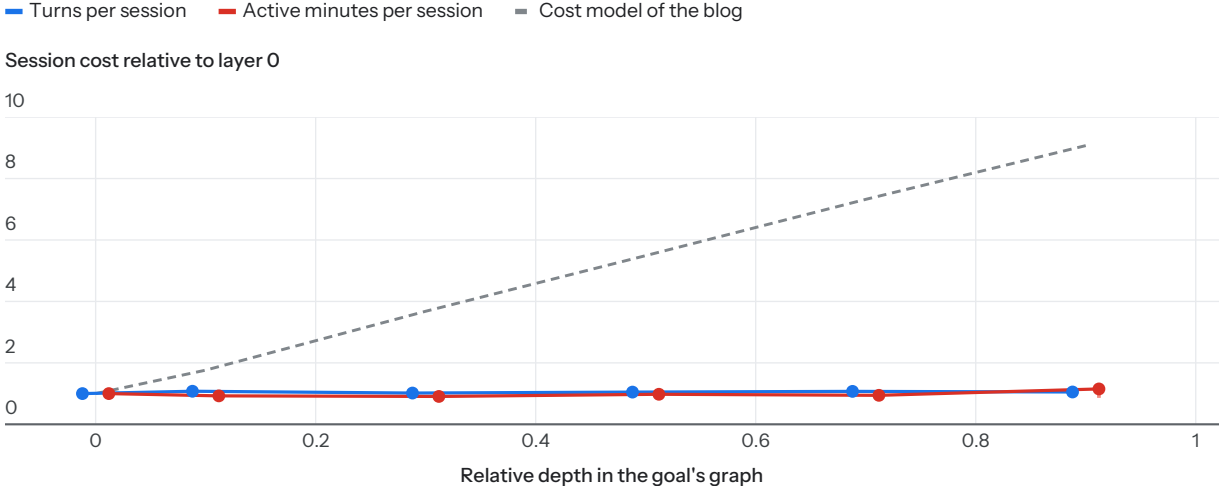
Figure 15: Turns and active minutes per computer-use session relative to the goal’s layer-0 sessions, by relative depth in the goal’s dependency graph, with 95% intervals, against the cost model of the blog. Real sessions cost about the same at every depth, while the cost model rises about ninefold.
