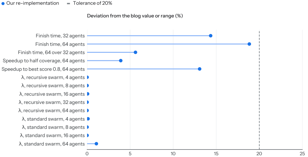
Figure 16: Deviation of our re-implementation from the blog for the 14 quantitative required checks, relative to the blog value or the nearest end of a blog range, over 256 families of 16 tasks. The fifteenth check, earlier coverage at every larger swarm, holds in all 256 families. Every deviation stays below the 20% tolerance.
