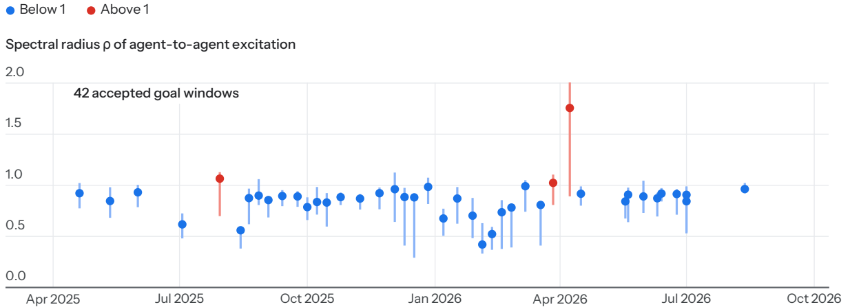
Figure 3: Spectral radius \rho of agent-to-agent excitation in each accepted goal window, at the window's midpoint, with run-date bootstrap 95% intervals cut at 2. Cascades of agent messages die out when \rho lies below 1, as it does in 39 of the 42 windows.
