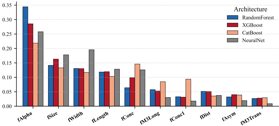
Normalized Mean SHAP
