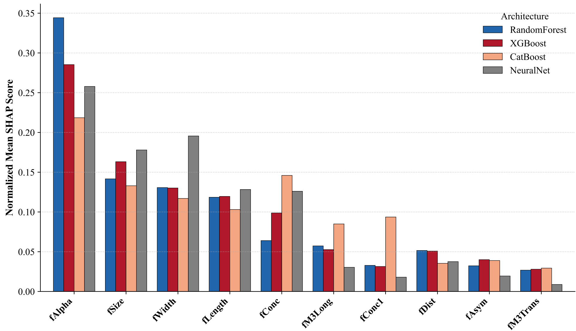
Feature Importance (Normalized SHAP) Across Architectures
