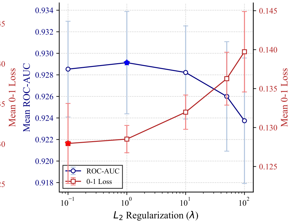
(f) L_2 Regularization ( \lambda )
