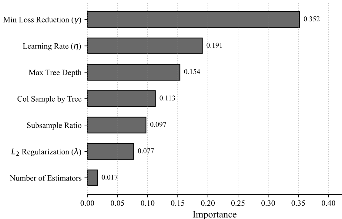
(b) Hyperparameter Importance
