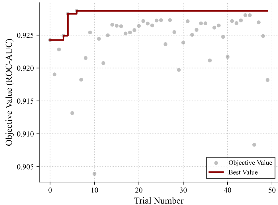
(a) Optimization History
