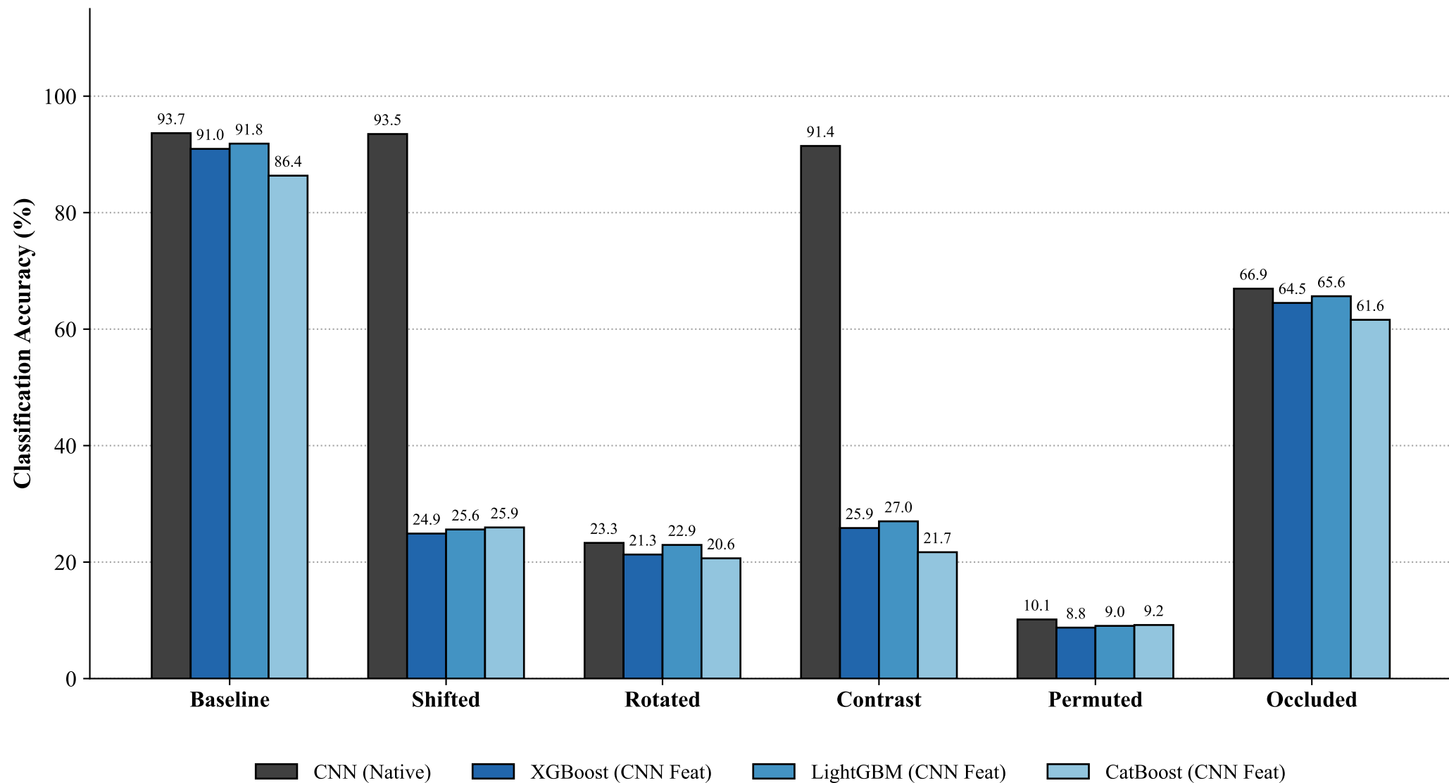
Native CNN vs. Hybrid (CNN-Feat) GBDTs
