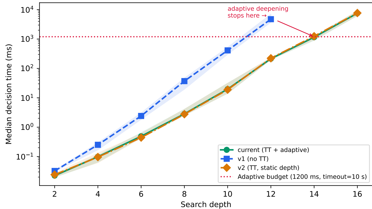
Decision time vs search depth (v1 → depth 12, v2/current → depth 16) shaded band = IQR, log scale
