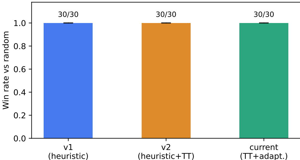
Version comparison (depth=8, N=30 games) \pm 1 binomial std error
