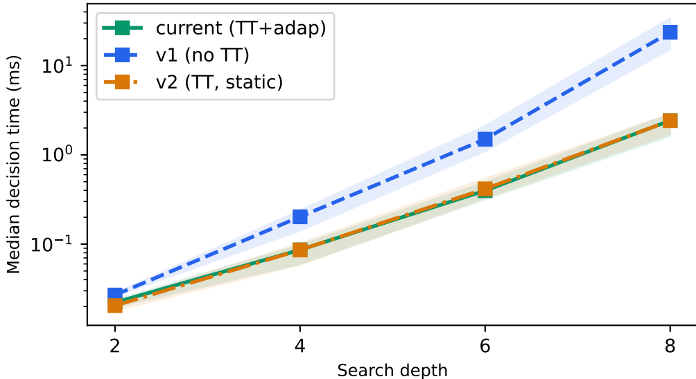
Decision time vs search depth (shaded band = IQR, log scale)
