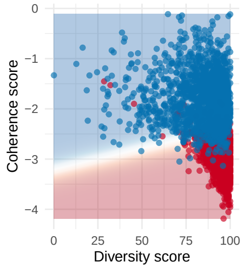
Top-p (0.95) Dataset: Book Accuracy: 0.9486
