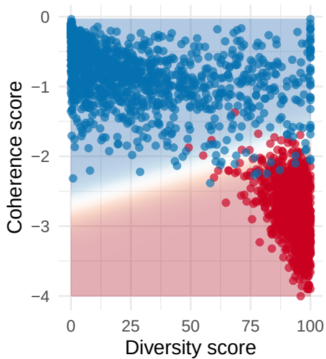
Beam Search (50) Dataset: Wikitext Accuracy: 0.9981
