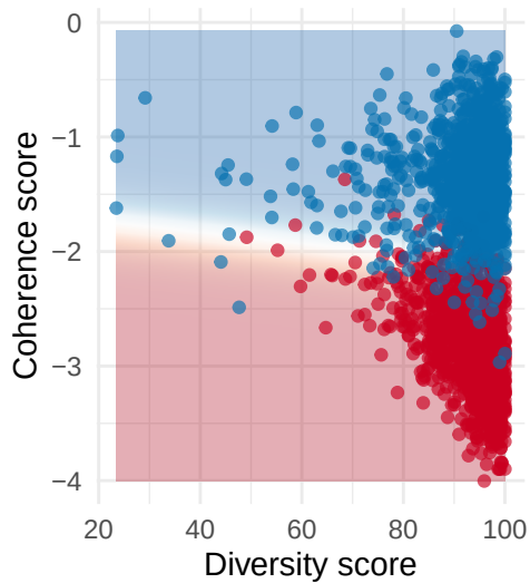
Temperature (1) Dataset: Wikitext Accuracy: 0.9637
