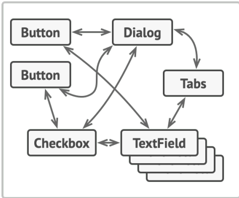
Profile Dialog
