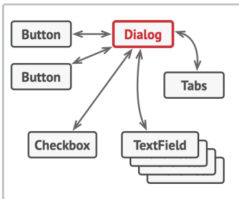
Profile Dialog
